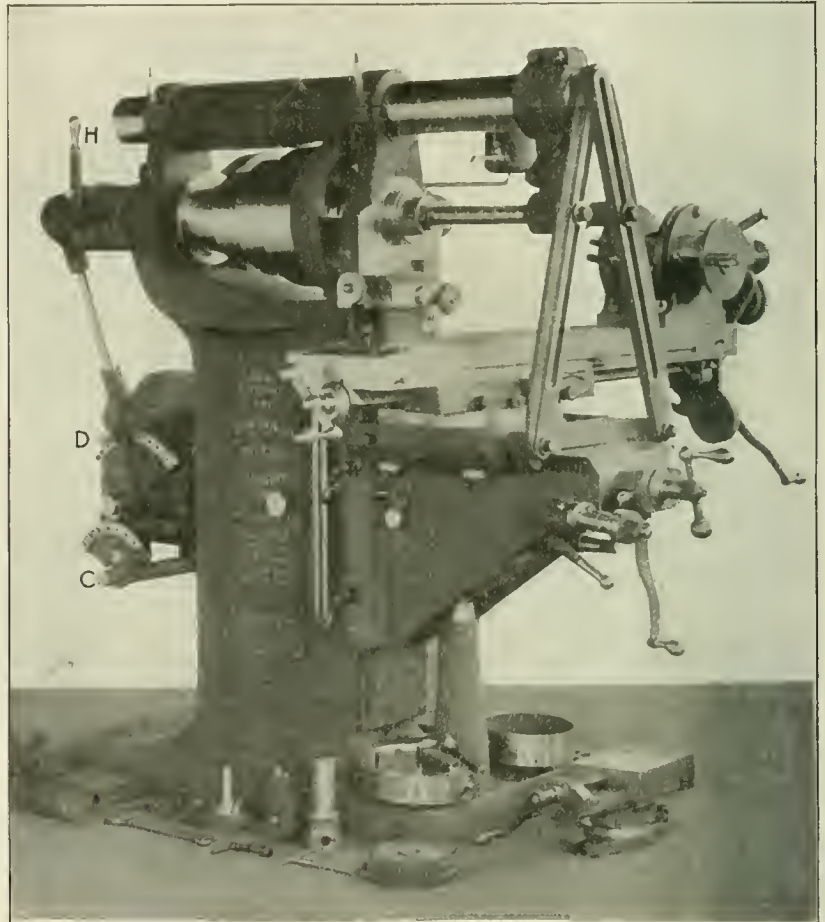
NEW CINCINNATI MILLING MACHINE.
